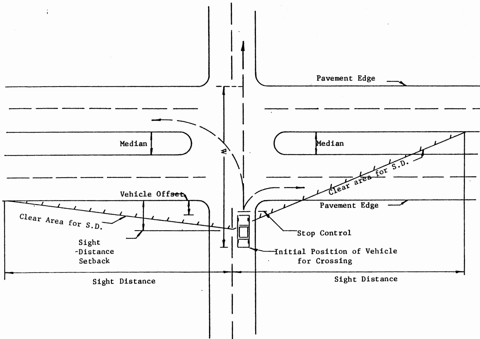
INTERSECTION CONFIGURATION
