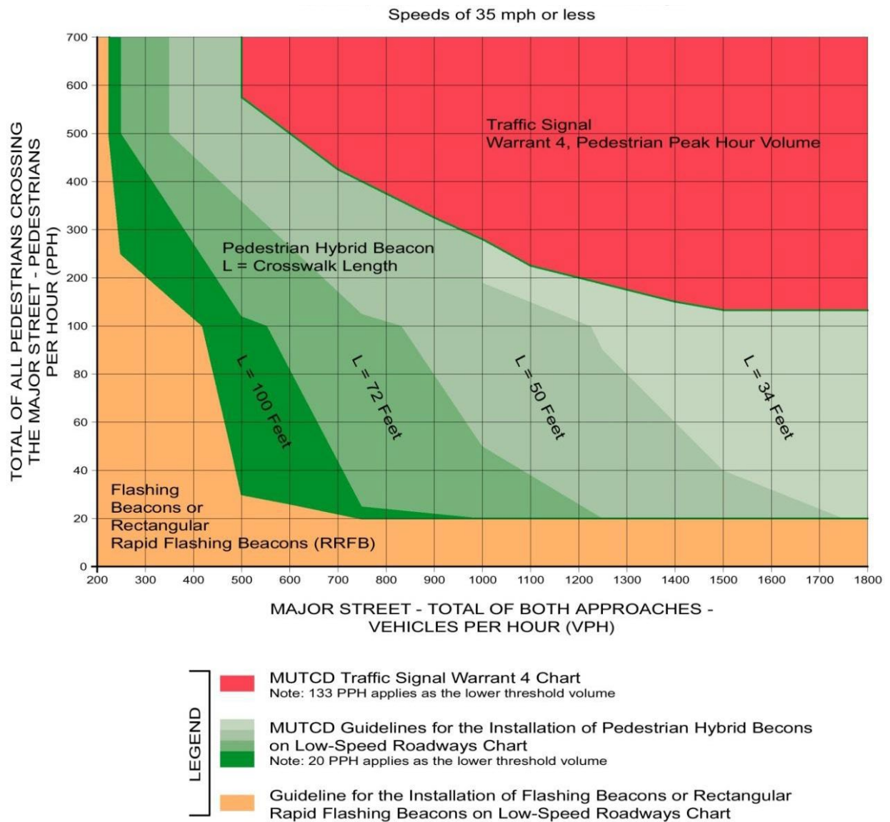
Figure 3.8-3. Guidelines for the Installation of Pedestrian Treatments on Low-Speed Roadways
