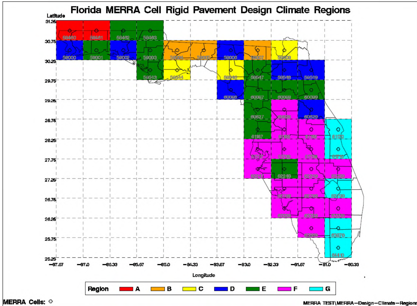
Figure 3.1 FLORIDA RIGID PAVEMENT DESIGN CLIMATE REGIONS
